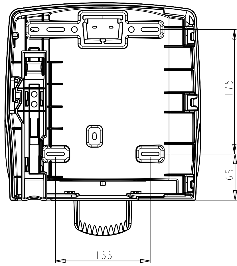
Drill pattern
