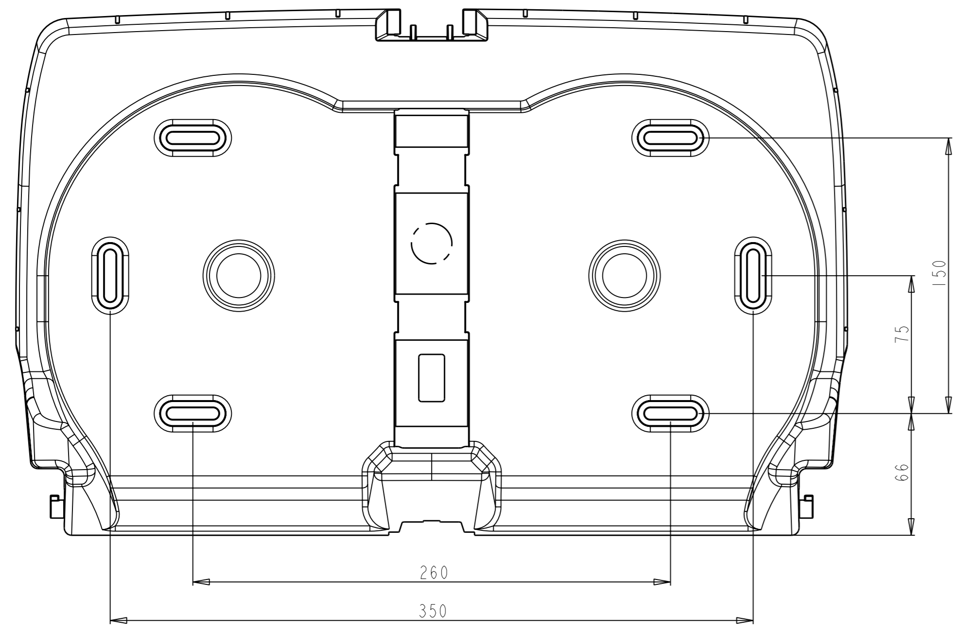
Drill pattern
